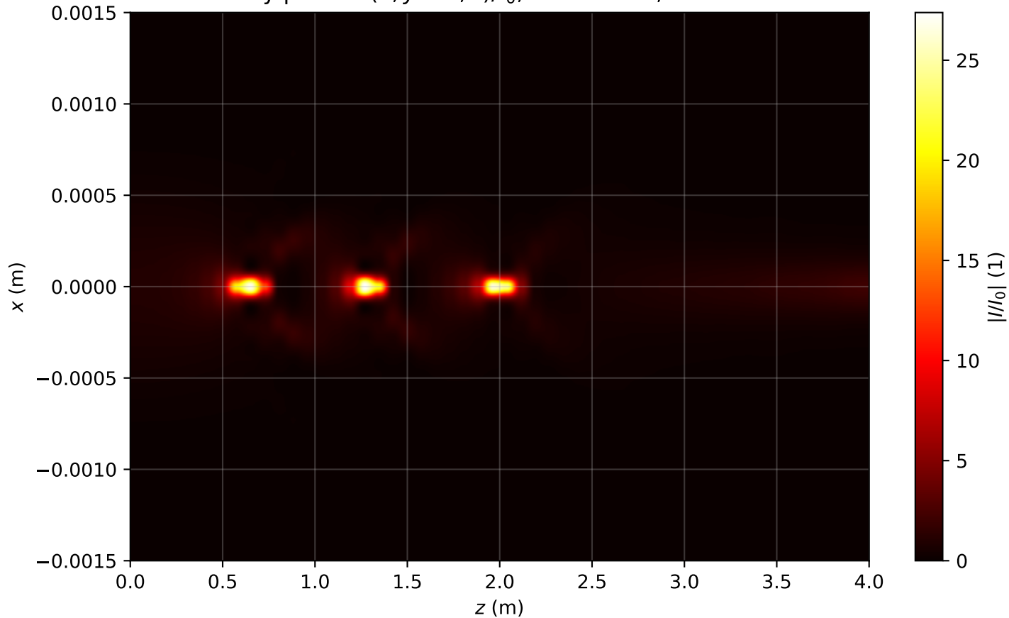
Intensity profile I(x, y = 0, z)/I_0 , P_{in}=4.0P_{cr} , artificial time
